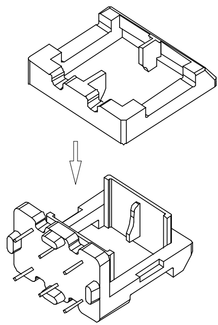
PART P-3502
